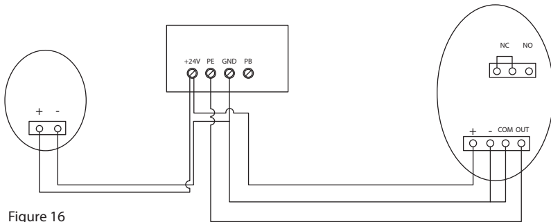
CONNECTION OF PHOTO BEAM/SWITCH CONTROL
